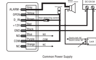
Common Power Supply
